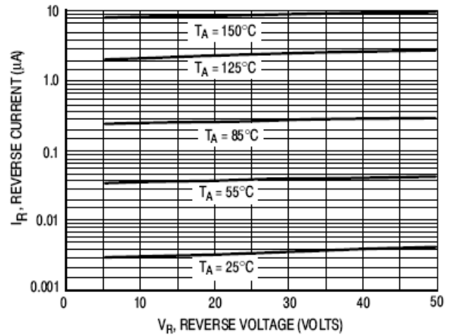
Figure 2. Reverse Current
