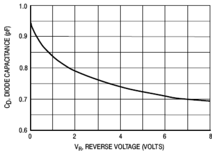
Figure 3. Diode Capacitance
